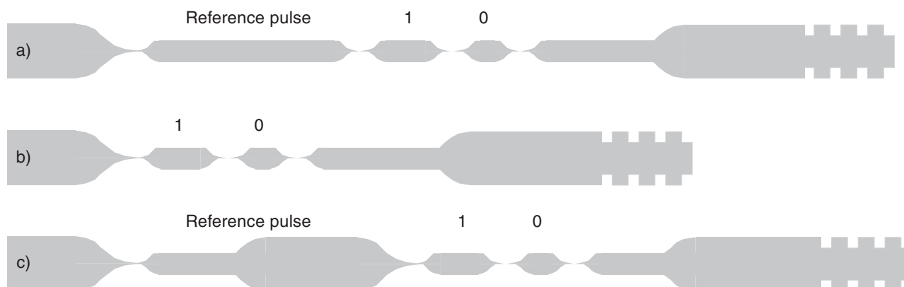
Figure 5-13. Long-leading-reference Protocol
