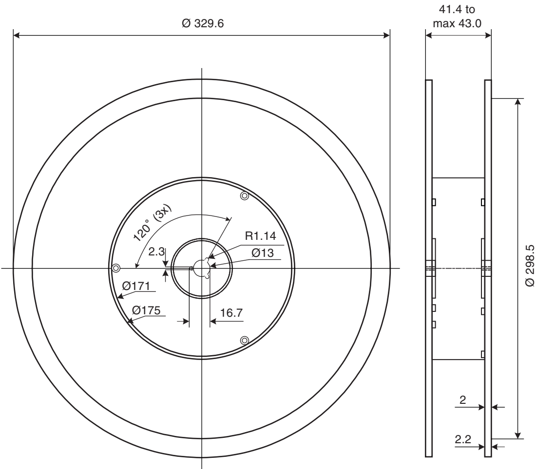
Figure 11-6. Shipping Reel for NOA3 Micromodule
