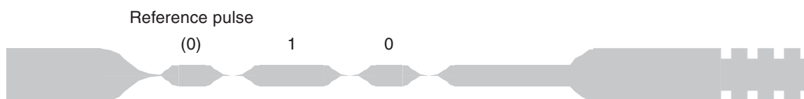
Figure 5-14. Leading-zero-reference Protocol
