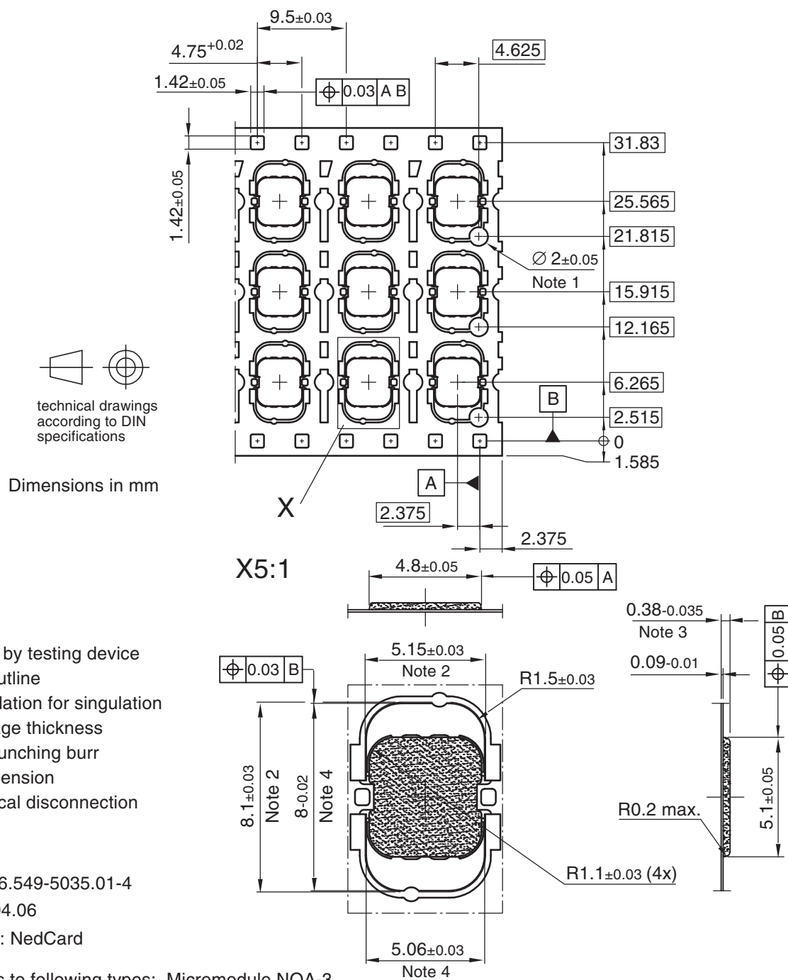
Figure 11-5. NOA3 Micromodule
